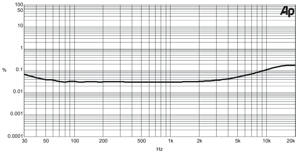
THD between 30Hz and 20 kHz
